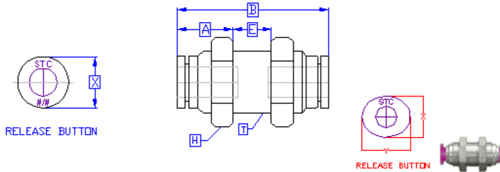
Bulkhead Union
